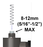
Figure 4. Quartz Sleeve Installation
